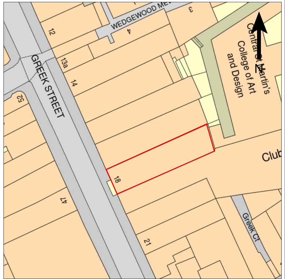
Location Plan 1:500
